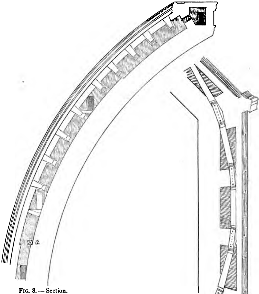
FIG. 8.—Section.
